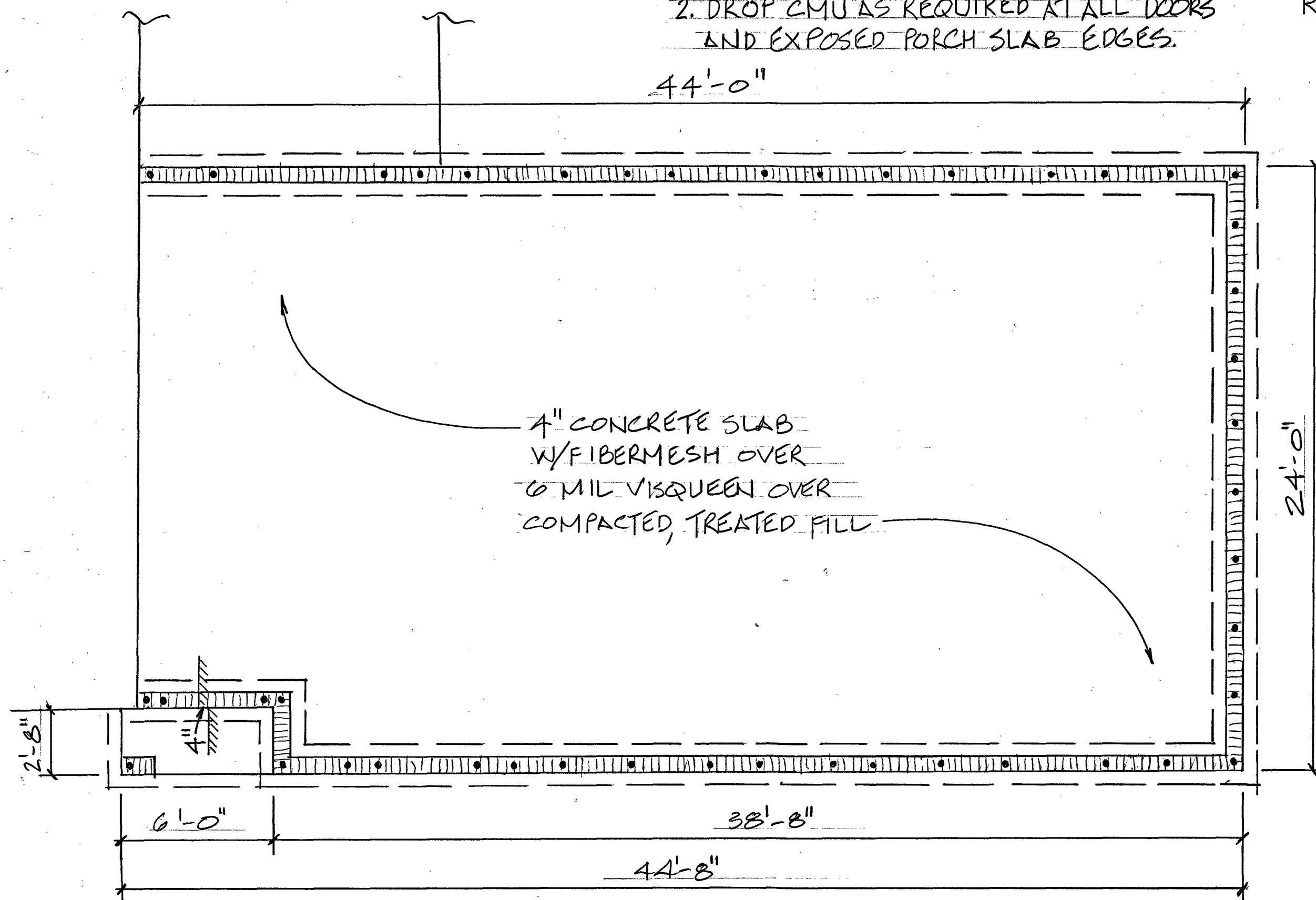
FOUNDATION PLAN
